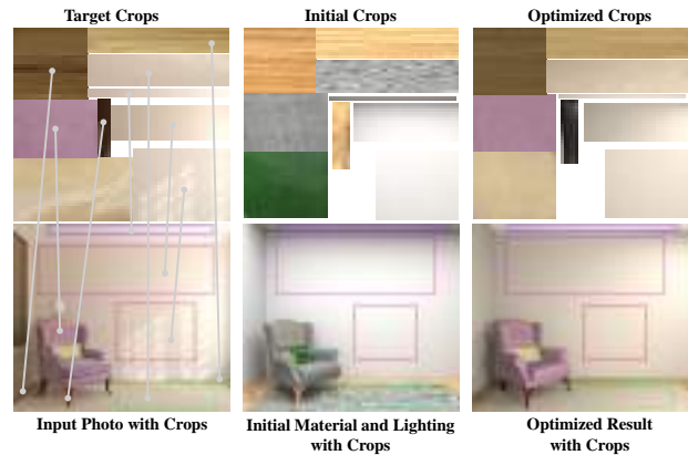
Figure 7: We visualize the crops from the input image, paired with rendered crops at initialization and during optimization. The optimized crops match the mean color and texture better comparing to the initialization. Losses based on Gram matrices of VGG layers are effective at matching texture in rectangular crops without need for pixel alignment.
