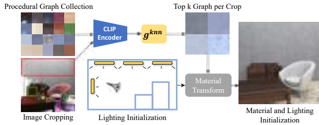
Figure 6: We use CLIP for zero-shot classification and ranking of materials, by comparing encoded thumbnails of our procedural materials with encoded input image crops. A user can optionally pick from top k matches. We further search for the best transform (scale and rotation) for the best texture match; this is done under the initial lighting. We keep some materials homogeneous (more detail in text).
